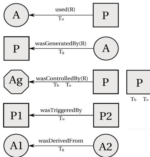
Figure 1: Edges and Usage of Timestamps in OPM. Source: [Moreau et al. 2011].
