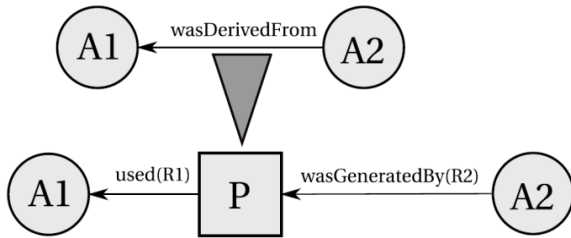
Figure 3: Process introduction. Source: [Moreau et al. 2011].
