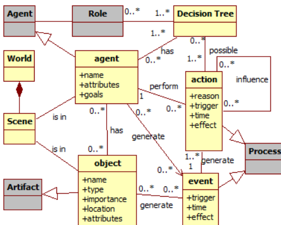
Figure 5: Data model diagram. Gray classes represents provenance classes.
