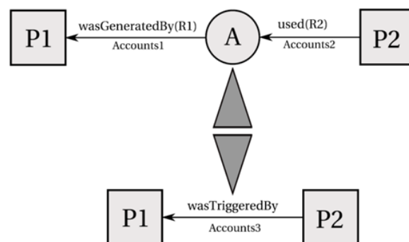
Figure 2: Artifact introduction and elimination. Source: [Moreau et al. 2011].
