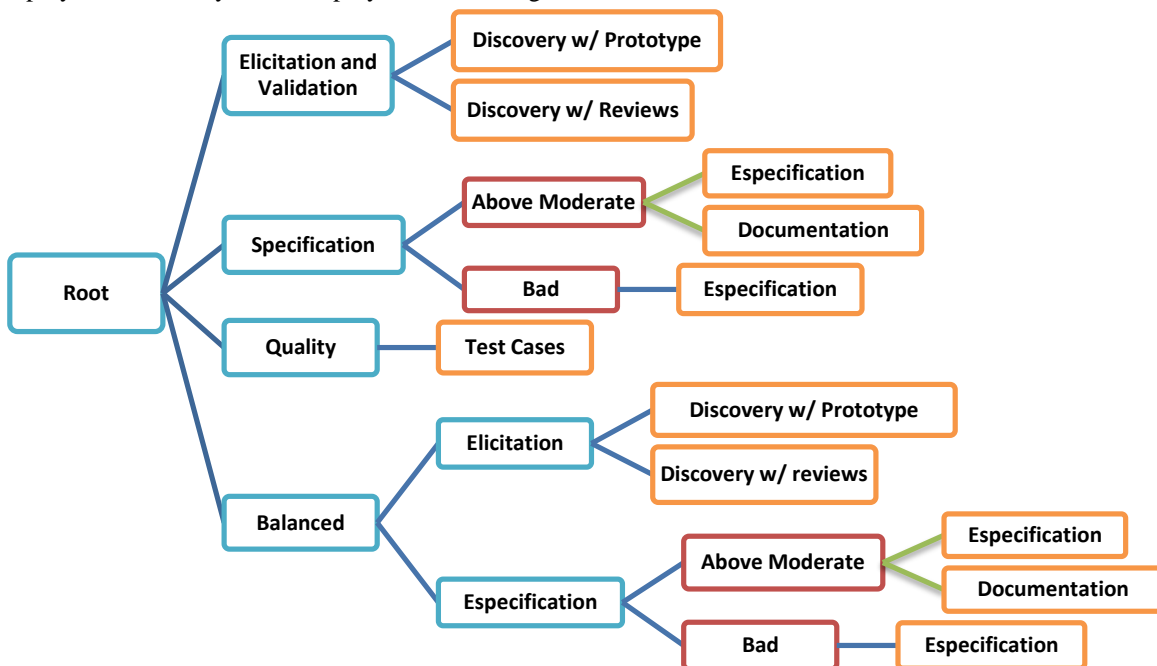
Figure 7: Analyst Decision Tree Example. Orange boxes represent end nodes (tasks). Red boxes are value evaluation. Green lines represent probabilistic paths and blue lines are decision paths.
