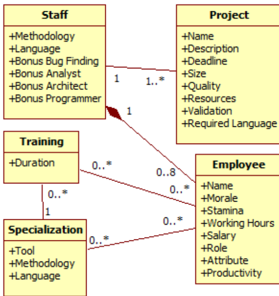
Figure 8: SDM's simplified class diagram. Adapted from [Kohwalter et al. 2011].
